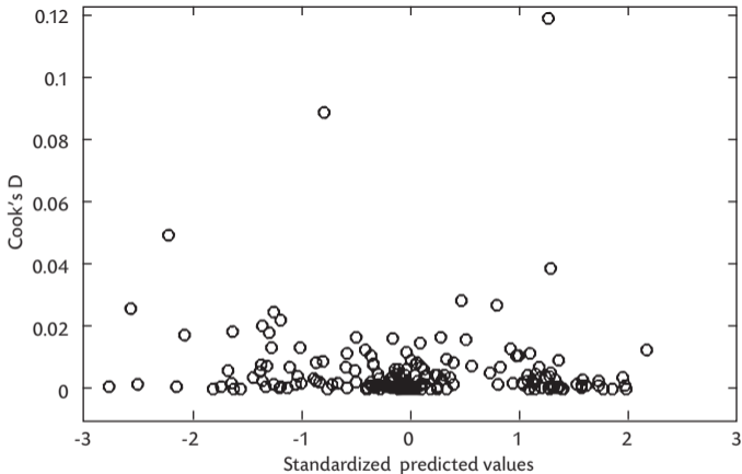
Figure 4.3 Scatter plot of Cook's D against standardized predicted (fitted) values for the model in Table 4.18, n = 189 .
