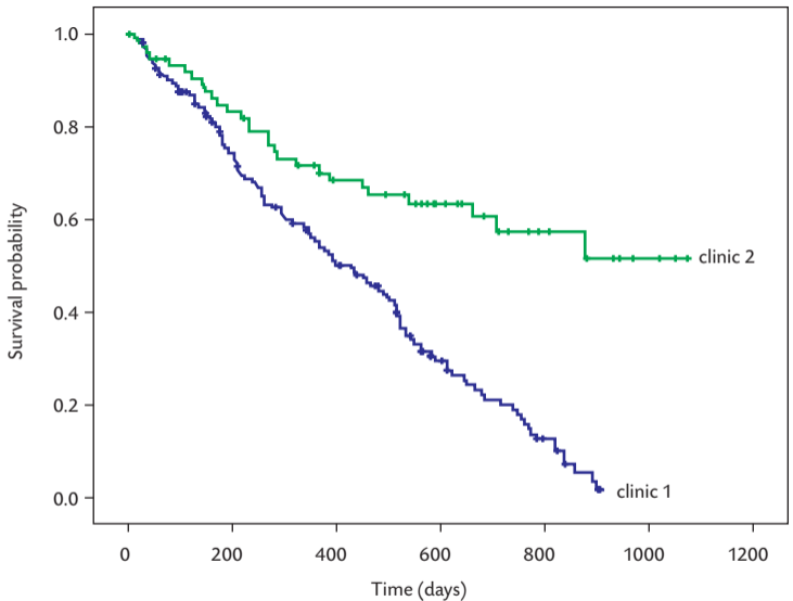
Figure 5.11 Kaplan-Meier plot comparing dropout from methadone treatment in two clinics. (Censoring times are marked on the curves.)
