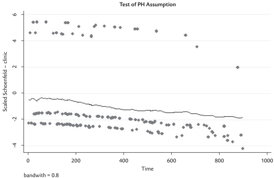
Figure 5.13 Plot of scaled Schoenfeld residuals for covariate CLINIC.
