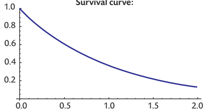
Survival curve:
