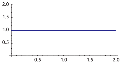
Hazard rate:
