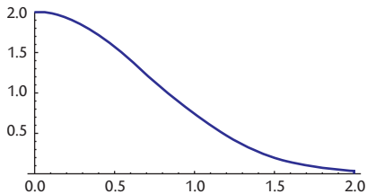
Figure 5.3 Hazard rates with corresponding survival curves.
