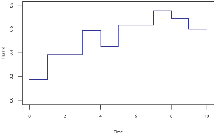
Figure 6.1 Example of a piecewise constant baseline hazard h_0(t) = h_{0k} when u_{k-1} < t \leq u_k .
