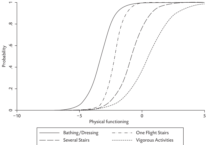
Figure 9.4 Physical functioning. Item characteristic curves for 2-PL. (Source: Rabe-Hesketh and Skrondal, 2008a.)
