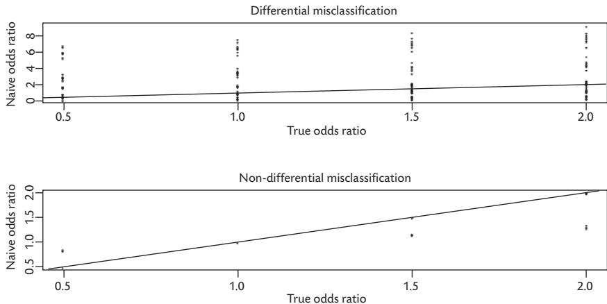
Figure 10.2 Plot of limiting value of naive estimator of the odds ratio versus true odds ratio in a 2 \times 2 table with either differential or nondifferential misclassification, over various combinations of sensitivity and specificity (see text). Line indicates where there is no bias.
